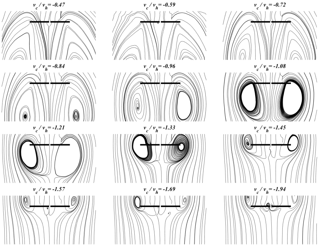
Figure S1: Streamline patterns for two rotors operating in steady axial descent at different normalized descent rates (4" rotors, S = 1.0 , 10314 RPM).
