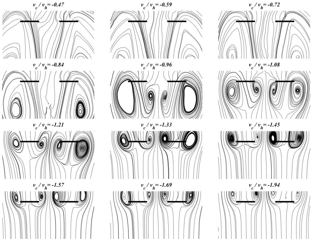
Figure S2: Streamline patterns for two rotors operating in steady axial descent at different normalized descent rates (4" rotors, S = 2.0 , 10314 RPM).
