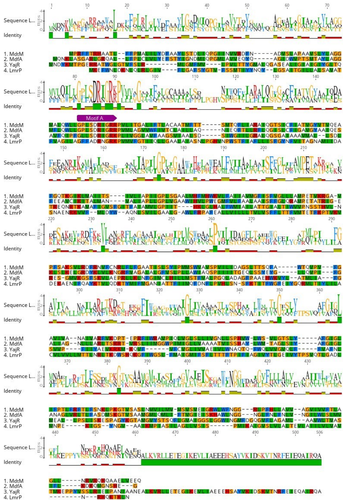
Supplementary Figure S1. Multiple sequence alignment of the Escherichia coli MFS multidrug efflux proteins MdtM, MdfA and YajR, and the Lactococcus lactis MFS multidrug efflux protein LmrP. The conserved, ten residue signature motif, Motif A, is annotated with the purple arrow.
