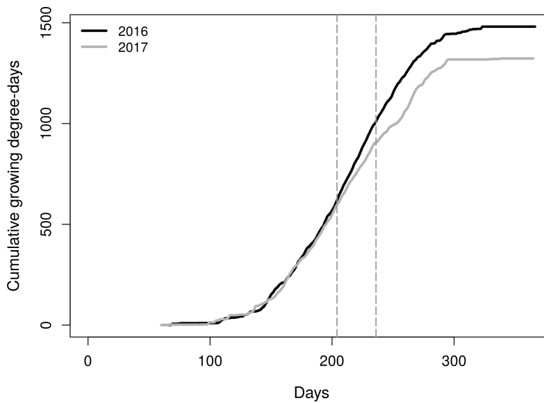
Fig. S1. Cumulative growing degree-days ( ^{\circ}\text{C d} ) versus day of year in 2016 and 2017, based on hourly temperature data from Dow Memorial Airport (MRCC 2018b) with initial day March 1 in both years. Dashed vertical lines indicate the earliest and latest seed collection dates in 2016 and 2017.
