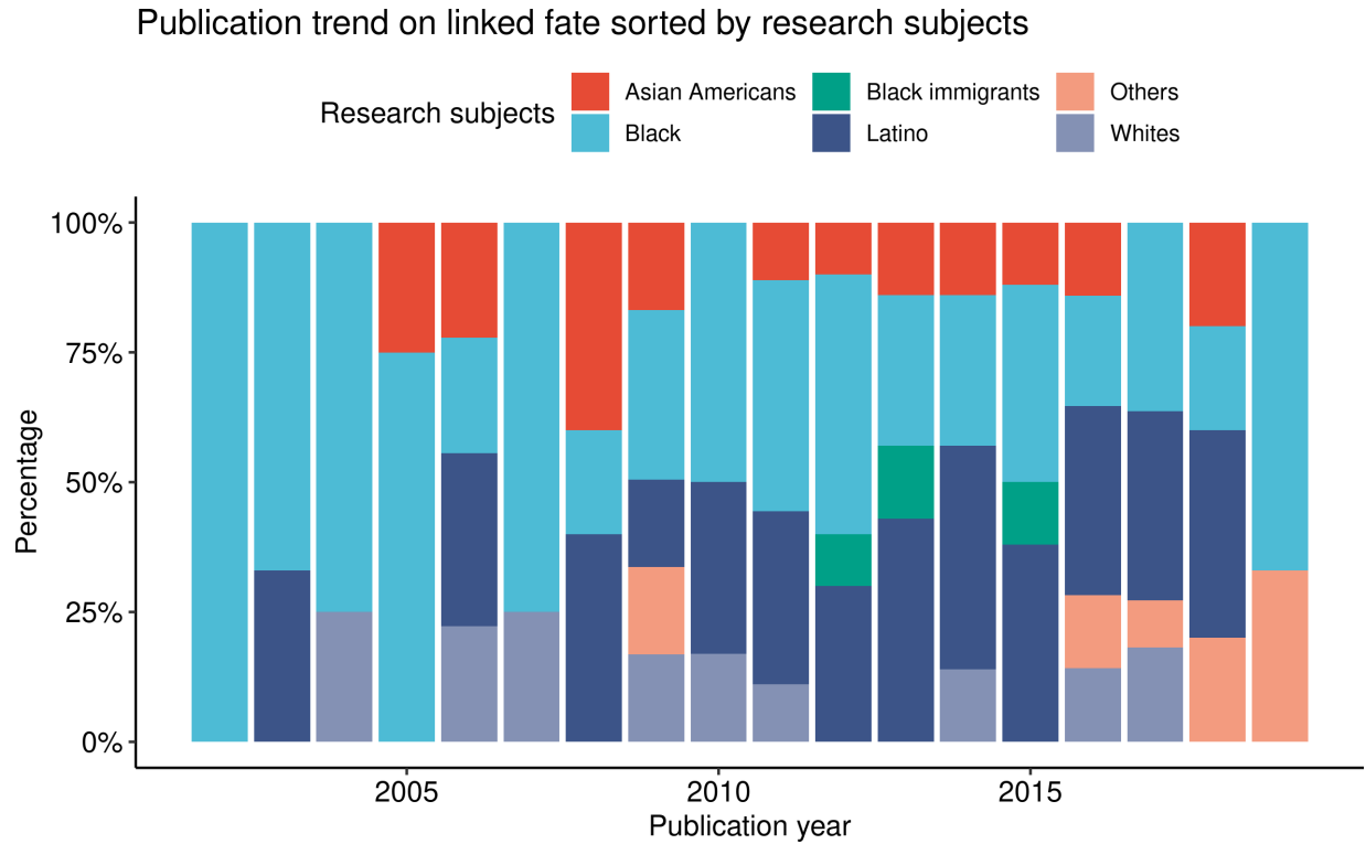
Figure A.1: Publication trend on linked fate sorted by research subjects
