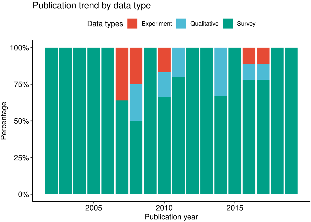
Figure A.2: Publication trend by data type
