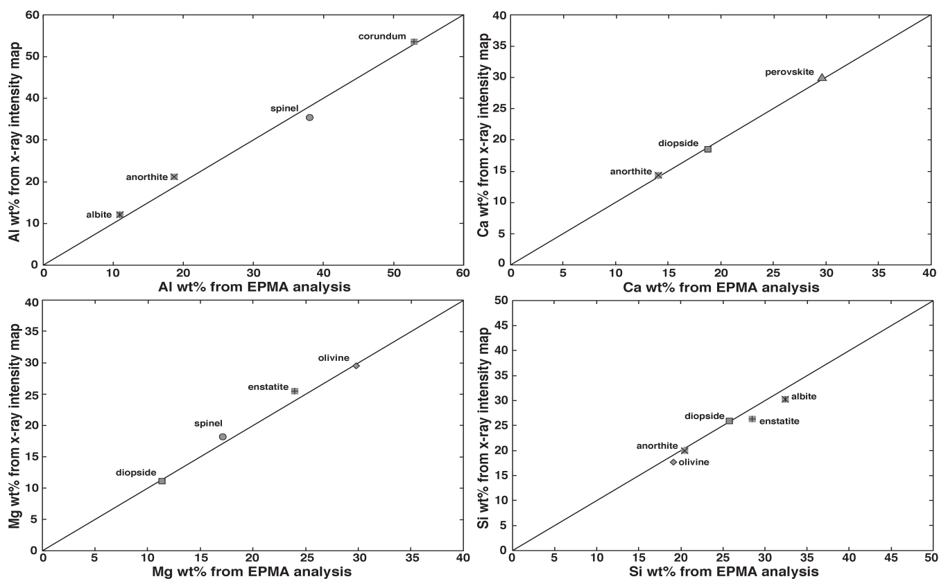
Supplementary Figure S3: Comparison of wt% determined from x-ray intensity maps using calibration curves, to that determined by EPMA quantitative point analyses with full PAP (ZAF) correction, for a suite of known standards. A 1:1 line is included for reference. All points are close to this line, indicating minimal differences between the two methods of concentration determination.
