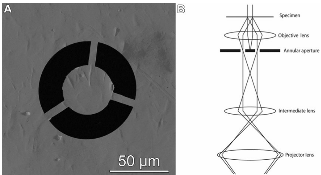
Supplementary Figure S1. (A) Secondary electron image of the annular aperture used in the experiment. (B) Schematic overview of the column of an electron microscope. The annular aperture is inserted in the back focal plane of the objective lens (adapted from Bals et al., 2006).
