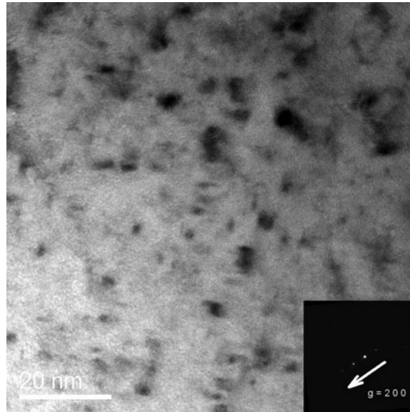
Supplementary Figure 1. BF image of displacement damage under two-beam condition, slightly “s +ve.” Inset: diffraction pattern showing g = \{200\} systematic row.
