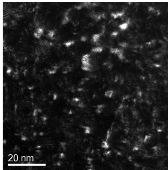
Supplementary Figure 2. DF image of displacement damage under two-beam condition, slightly “s +ve.”
