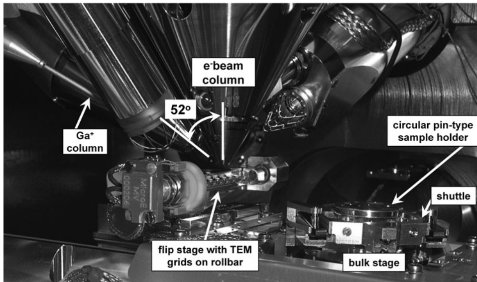
Supplementary Figure 1. Optical image of the inside of the Helios 400s DB-FIB chamber with both bulk and flip stages labeled.
