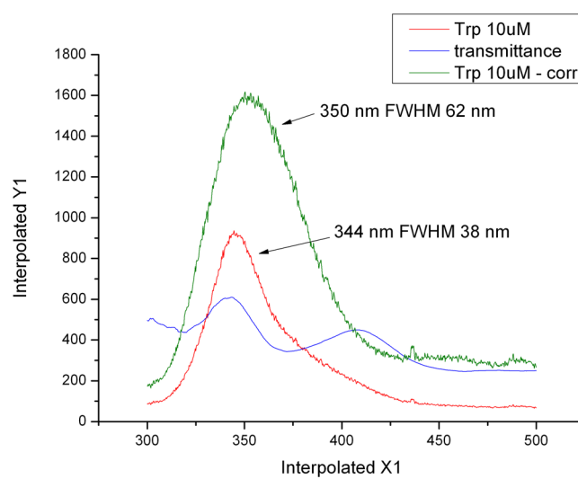
Supplementary Figure 1. The spectral corrections in the UV range do not show great modifications in the tryptophan region.
