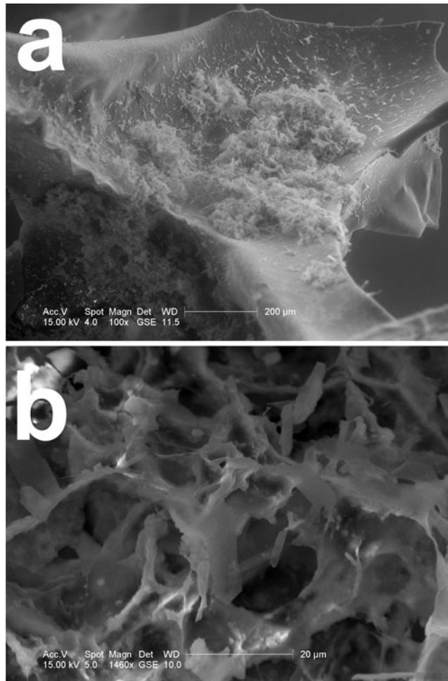
Supplementary Figure 1. The image of bacterial biofilm immobilized on OCPM visualized with environmental SEM use. This kind of microscopy allowed to show our bioreactor—a wet object, in micro-scale without any treatment before imaging. That images confirmed our data obtained with SEM use with material lyophilization (Fig. 6G,J–L) as a step of preparation.
