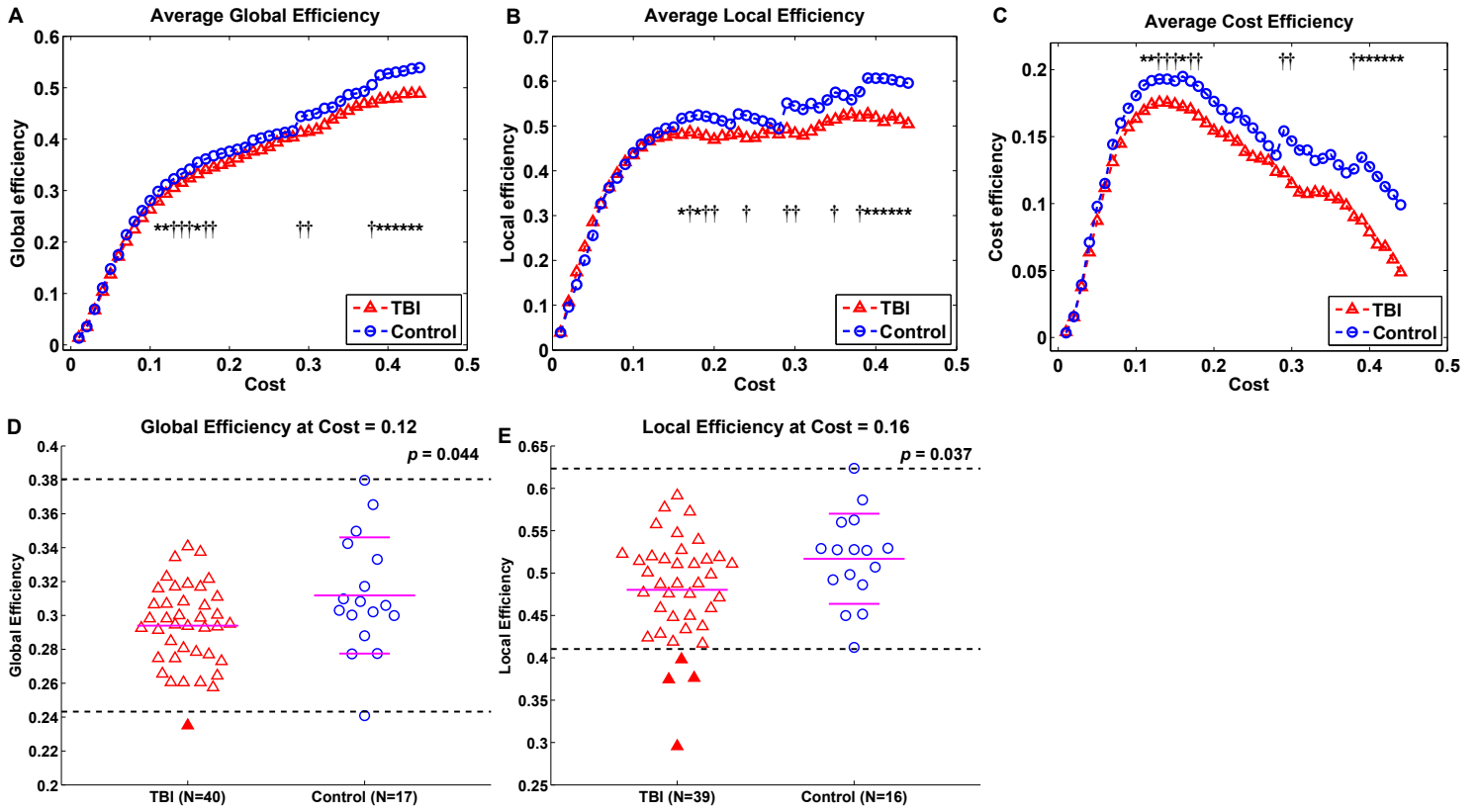
Fig. S12. Global, local and cost efficiency of the TBI group and the controls without global signal regression. (A)-(C): Average global, local and cost efficiency as a function of network cost, respectively. Note that, to reliably perform group analyses, we limited ranges of network cost (from 0.01 to 0.44 in step size of 0.01) to include N \geq 5 per group. (D), (E): Scatter plots for global and local efficiency at network costs of 0.12 and 0.16, respectively. See Fig. 4 for the details of the scatter plots.
