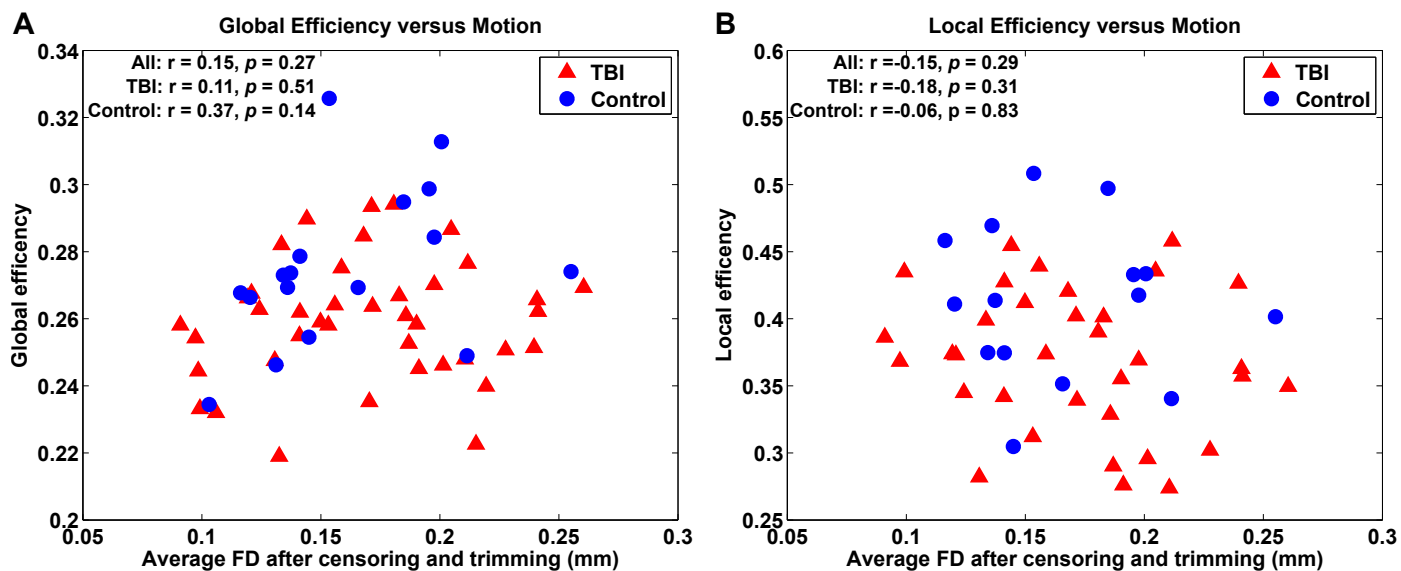
Fig. S1. Average framewise displacement (FD) of each participant after motion censoring and trimming versus the average global (A) and local (B) efficiency at network costs of 0.12 and 0.15, respectively. The r-values are the Pearson correlation coefficients.
