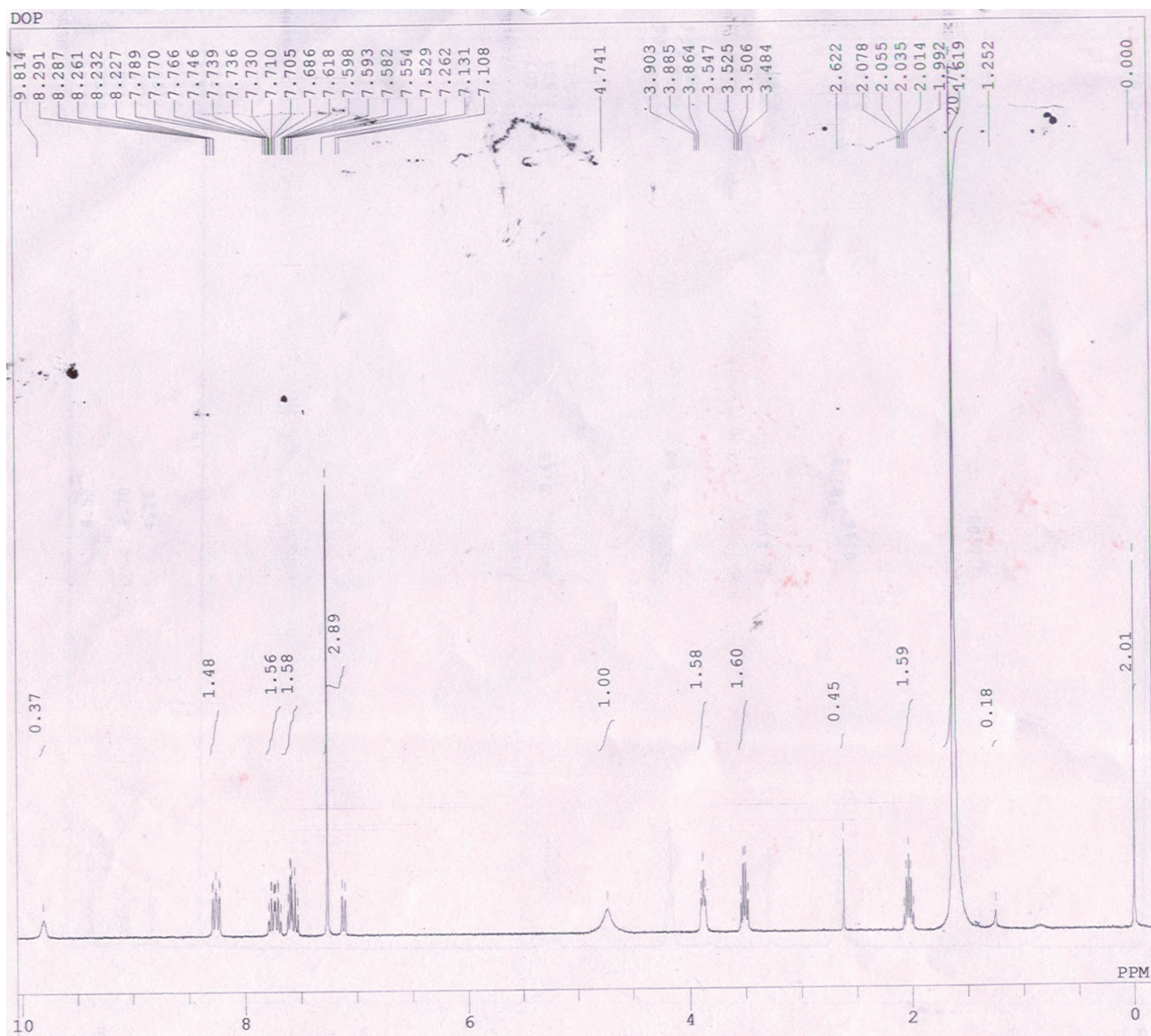
Fig. S. 1 H NMR spectrum of 1-(3-hydroxy-propylamino)-9,10-anthraquinone compound.
