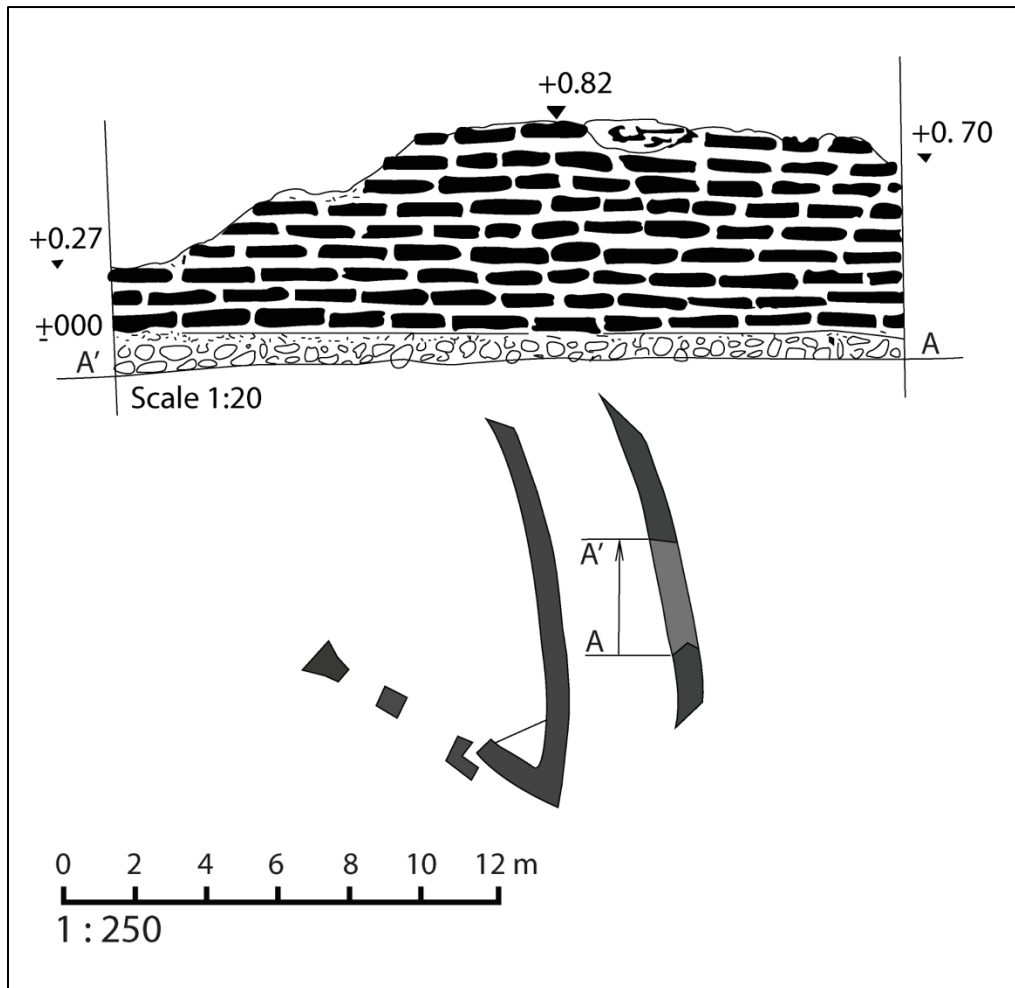
Suppl. Fig. 1. Plan and elevation drawing of the curved wall (Fig. 4: 002) northeast of the baths. (Drawings by P. Naipi.)
