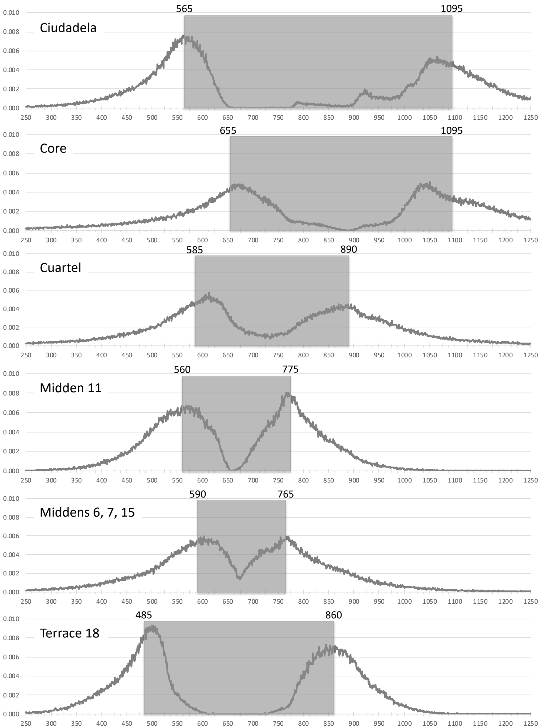
Supplemental Figure 1. Bayesian modeling of start and end dates for different sectors of La Quemada (at one sigma confidence level).
