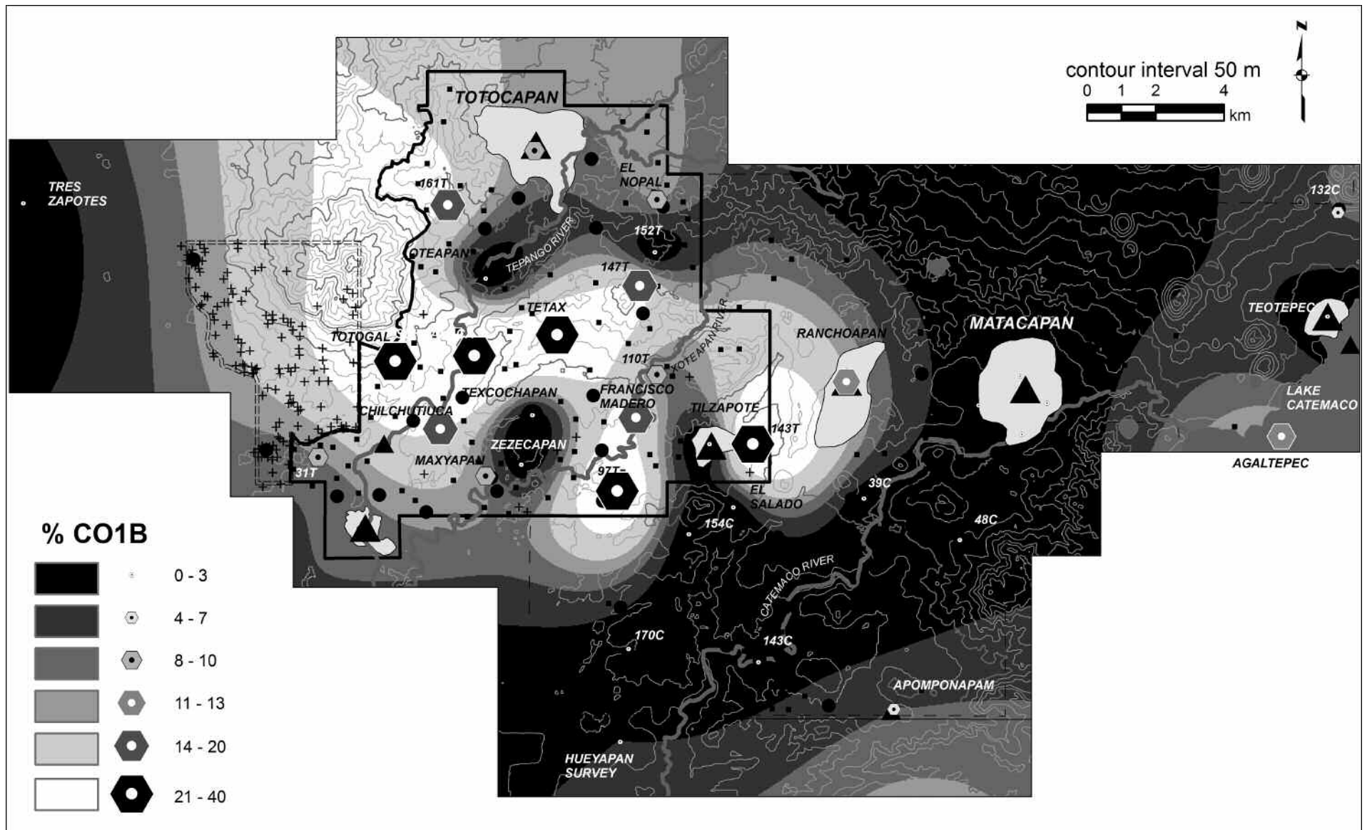
Supplemental Figure 3. Map showing the distributions of the CO1B chemical group. Choropleth zones are defined by natural breaks in the data.
