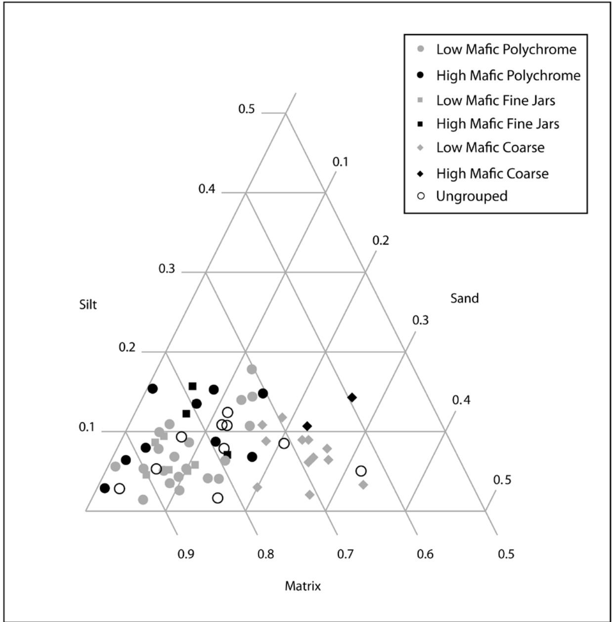
Supplemental Figure 2. Ternary diagram plotting ceramic samples based on ratios of silt to sand to matrix.
