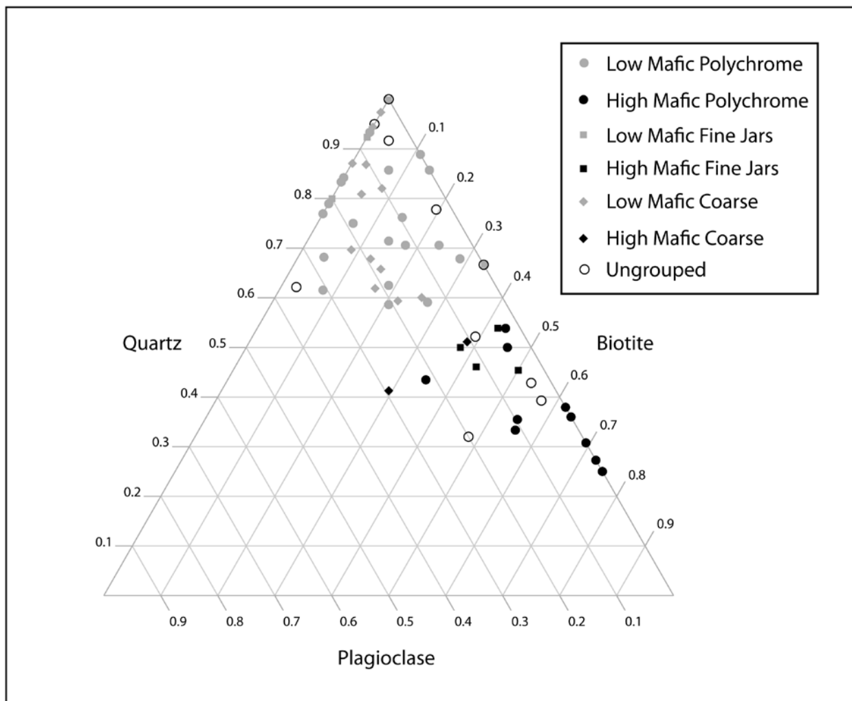
Supplemental Figure 1. Ternary diagram plotting ceramic samples based on mineral ratios that distinguish specimens with high vs. low mafic concentrations.
