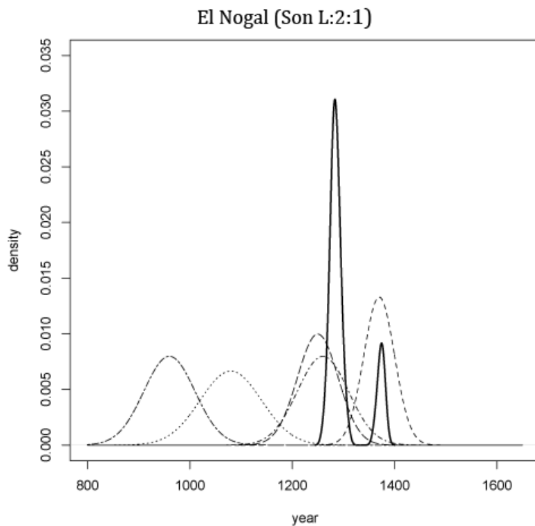
Supplemental Figure 3. Probability distribution of dates from Teonadepa and El Nogal. The solid lines are calibrated ^{14}\text{C} dates; the dashed lines are luminescence dates. Note that the slightly earlier termination of occupation at El Nogal is likely due to chance sampling and the fact that several dates are maximum ages (i.e., the samples were drawn from below the context of interest). Both sites contained several proto-Hispanic artifacts. The cross-dating of rare painted ceramics also suggests contemporaneity.
