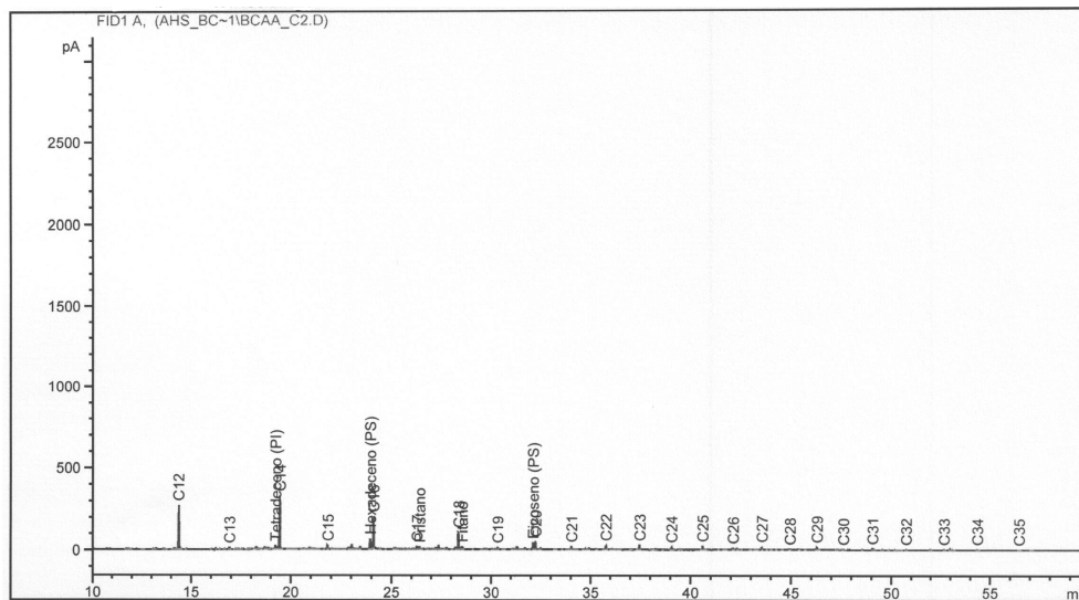
Distribution of n-alkanes in soil (station T11 with high UCM and T1 without UCM) and melt water stream sediments (station C2) near the Artigas Research Station (BCAA).
