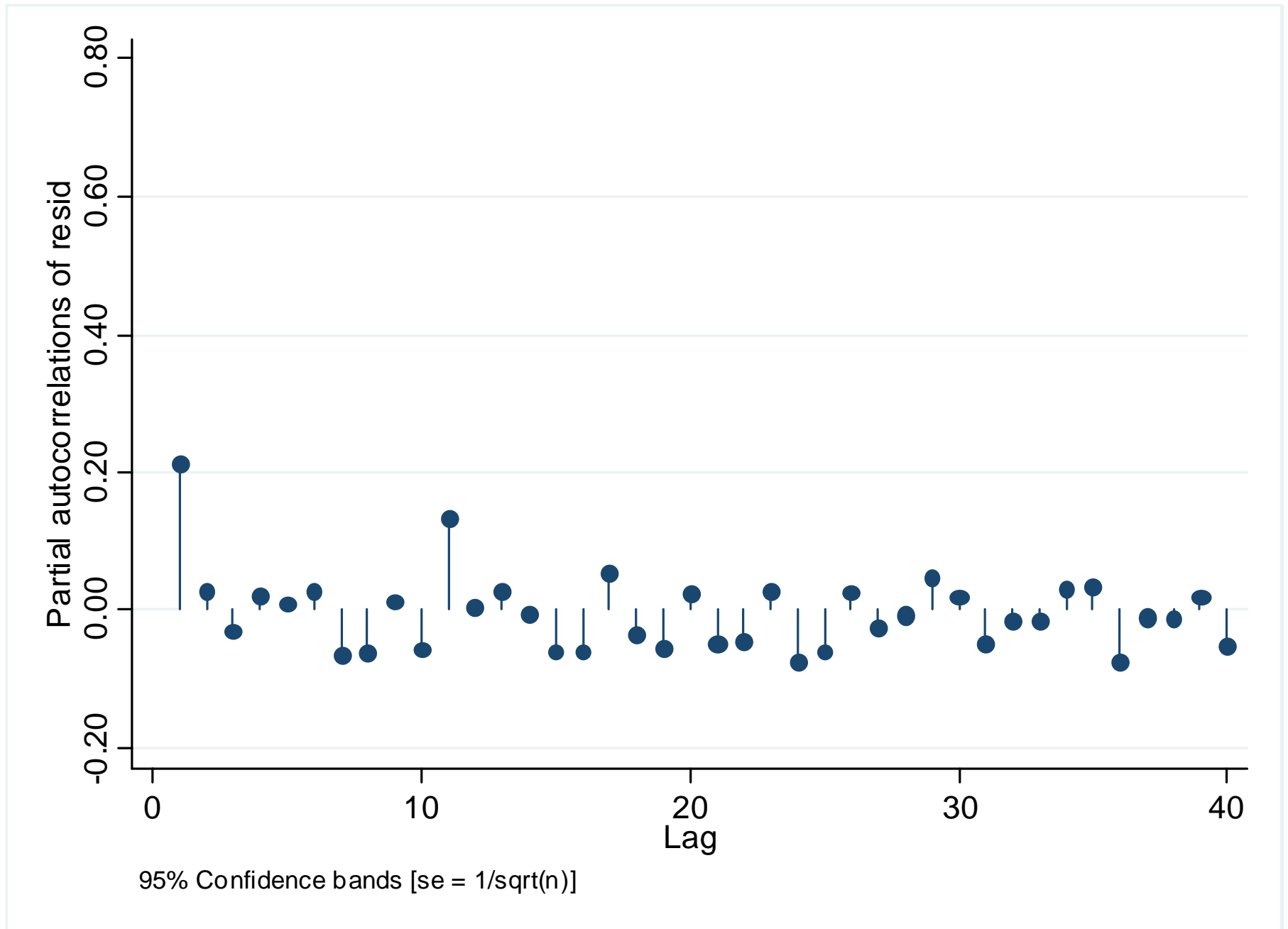
Fig. S1. (c) Partial autocorrelation function of the residuals.
