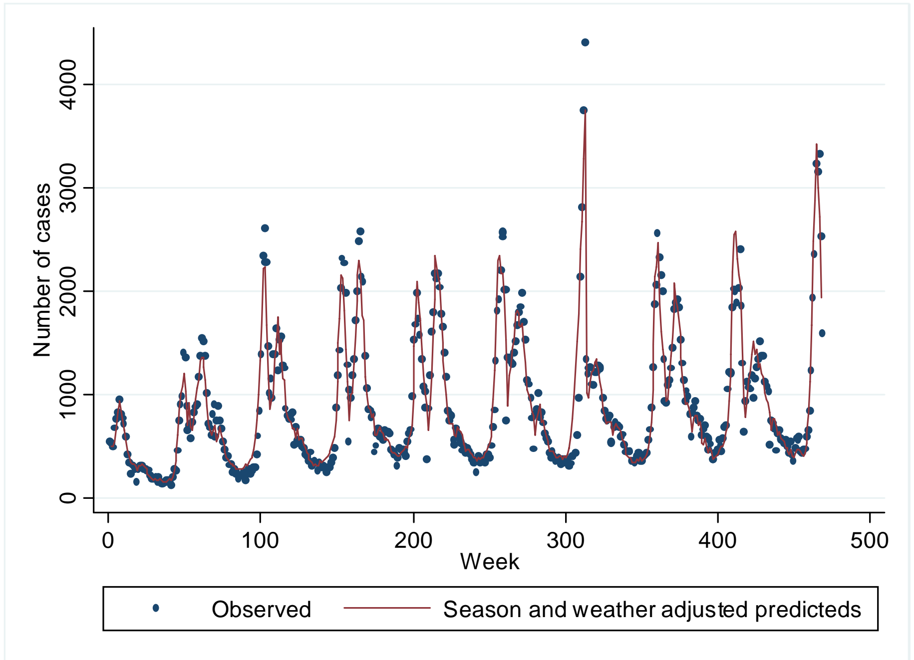
Fig. S1. (b) Predicted and observed time-series plots.
