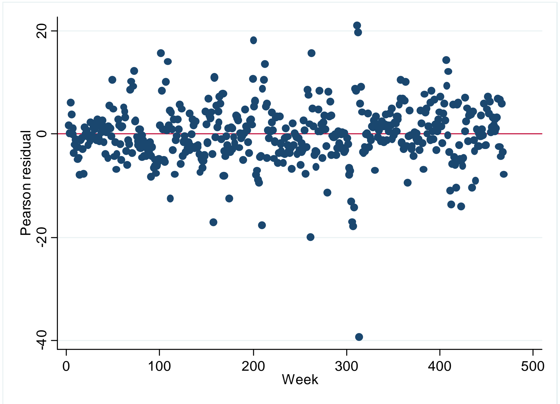
Fig. S1. (a) Plots of model residuals.
