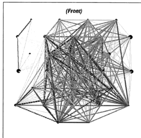
Figure 2 (Mayer-Kress). Frequency (point size) of short-term 40-Hz events at 31 electrodes and frequency (line thickness) of coincidences (simultaneous 40-Hz events between pairs of electrodes). Note that some far apart locations “communicate” much more intensely than some neighboring sites. (See Mayer-Kress 1994 for details; data courtesy of W. Miltner.)
