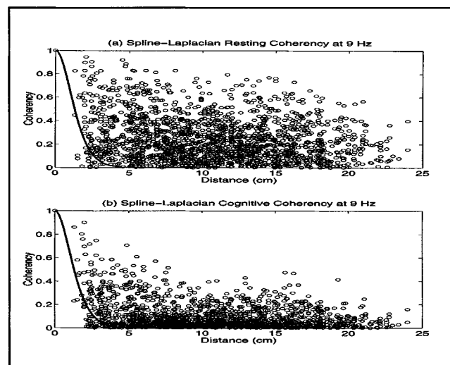
Figure 2. High-resolution coherence as a function of interelectrode separation. The same 60-channel raw data used in Figure 1 were first passed through the New Orleans spline – Laplacian algorithm to estimate potential distribution on the dura surface, thereby minimizing volume conduction distortion and eliminating reference electrode contributions to coherence estimates (Nunez 1995; Nunez et al. 1997; 1999). Large resting Laplacian coherencies were obtained at 9 and 10 Hz, but not at other frequencies. The largest coherence decreases between resting are cognitive states involved frontal-to-frontal sites. Melbourne dura image methods yielded similar coherence plots. The solid line is the analytic estimate of scalp Laplacian coherence expected from the same uncorrelated, radial dipole sources used to plot the solid line in Figure 1. Because high resolution methods filter out the longest waves from the spatial spectrum of source activity (which we are not able to distinguish from volume conduction), high-resolution coherence may underestimate actual source coherence (Nunez et al. 1997; 1999).
