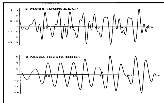
Figure 6. Solutions of the system of global mode equations (22), derived in the Appendix. The system consists of 5 coupled, second-order ordinary differential equations, each with about 40 mode-coupling terms. The vertical axis represents normalized synaptic action density at centimeter scales. The horizontal axis is normalized time [time (sec)/ \tau_g ], where \tau_g = 1/\lambda v is the characteristic global delay time, apparently in the 6–16 msec range based on long corticocortical fibers. If \tau_g = 10 msec, the period shown is 1 sec and dominant frequencies are in the 11-Hz range. The upper plot is the sum of modes \Phi_n(t) , n = 1, 5 , crudely representing dura potential. The lower plot is the same solution, but with modes n = 3, 4 , and 5 removed to simulate crudely spatial filtering by the head volume conductor between dura and scalp. Other numerical solutions (not shown) indicate that increases in the linear feedback parameter B cause amplitudes to increase with minimal frequency changes for small to moderate B . Large B values produce solutions with larger amplitudes and lower frequencies. The parameters for this numerical solution are B = 2.2 , A = 0.0667 , k_n^2 = 1.5, 1.95, 2.70, 3.75, 5.10 ( n = 1, 5 , consistent with the rectangular geometry discussed in the Appendix).
