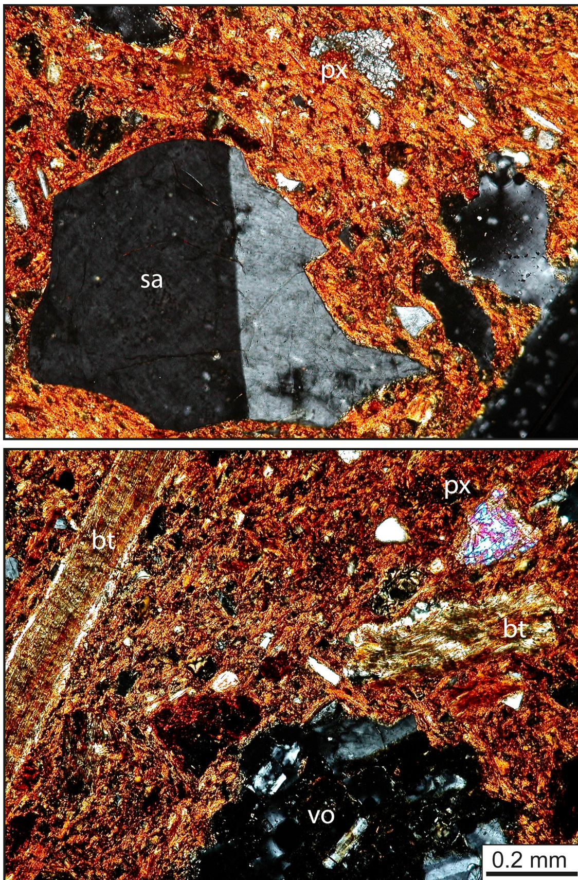
Online Fig. 1: Microphotographs of Gloucester TF214, sample RTS-211 (crossed polars); bt = biotite, px = clinopyroxene, sa = sanidine feldspar, vo = volcanic rock. (Photograph: Claudio Capelli)
