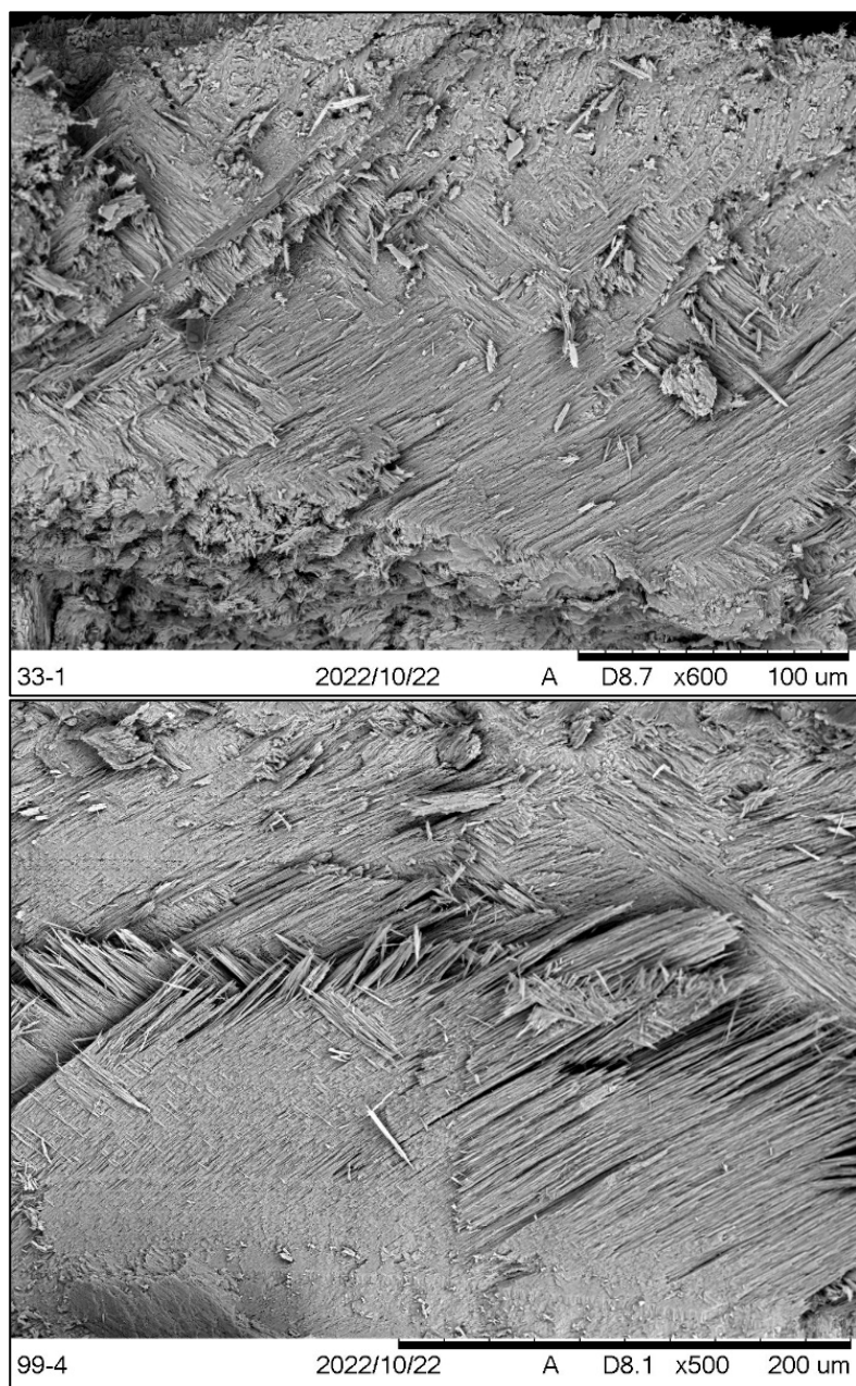
Supporting Figure 1. SEM images of shell fragments from Layer 5 (top) and Layer 3C (bottom) showing crossed-lamellar layers.
