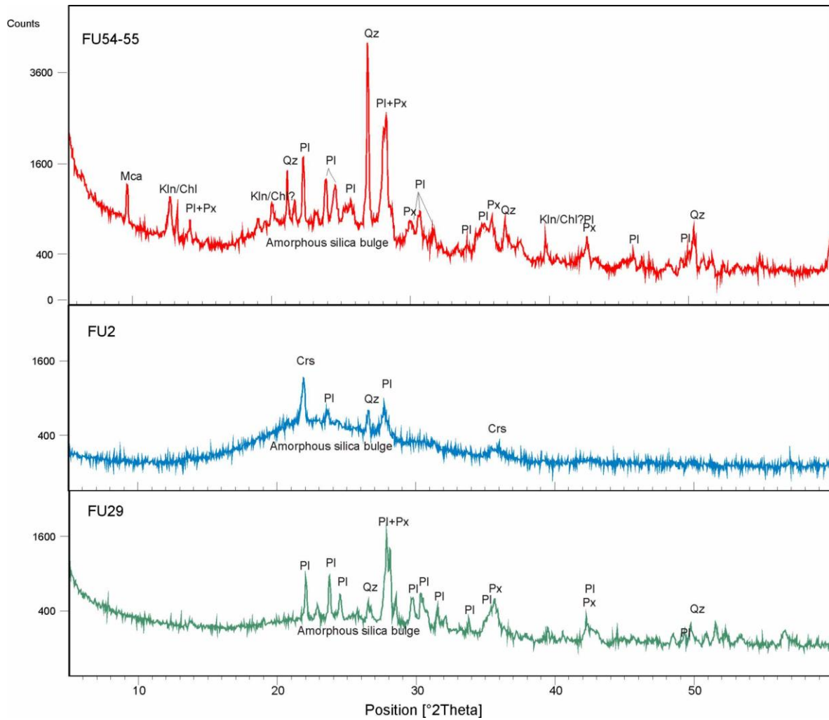
Figure S1. Characteristic X-Ray Diffraction Patterns for sediments of Lake Futalaufquen sequence (FU54-55), and two tephra layers (FU2 and FU29).
