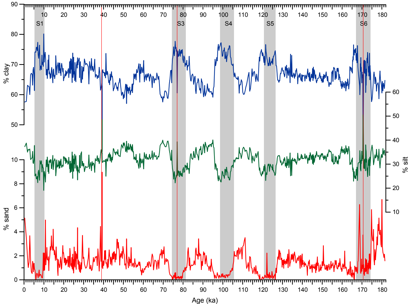
Fig. S3: Sand, silt and clay percentages within the terrigenous sediment fraction of core SL99. Grey shaded areas mark sapropels, red lines indicate ash layers.
