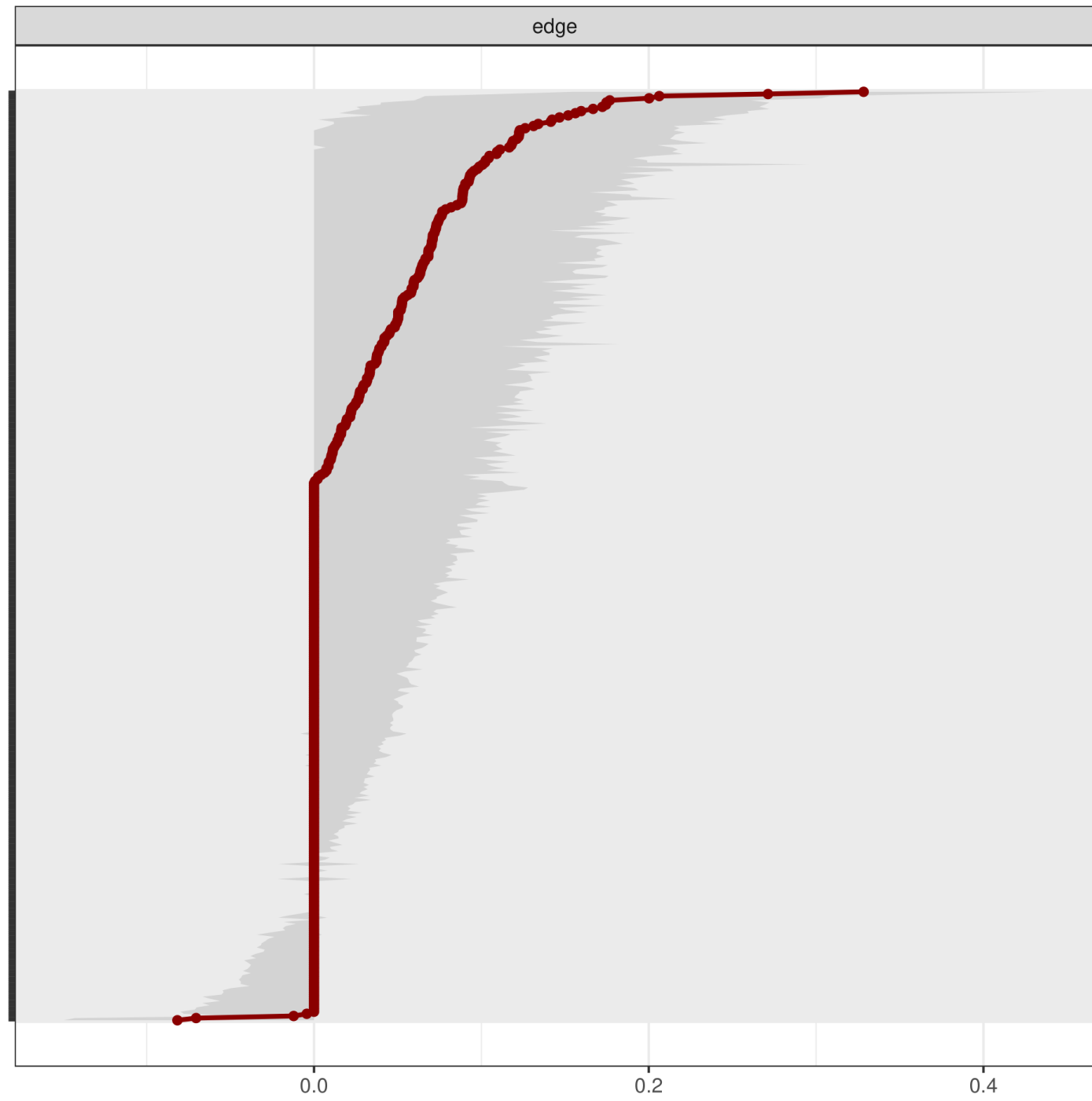
Fig. S14. Bootstrapped Confidence Intervals of edge-weights for the PCBD/PTSD networks. Red lines represent edges, ordered by edge weight magnitude, and the gray areas represent their bootstrapped CIs.
