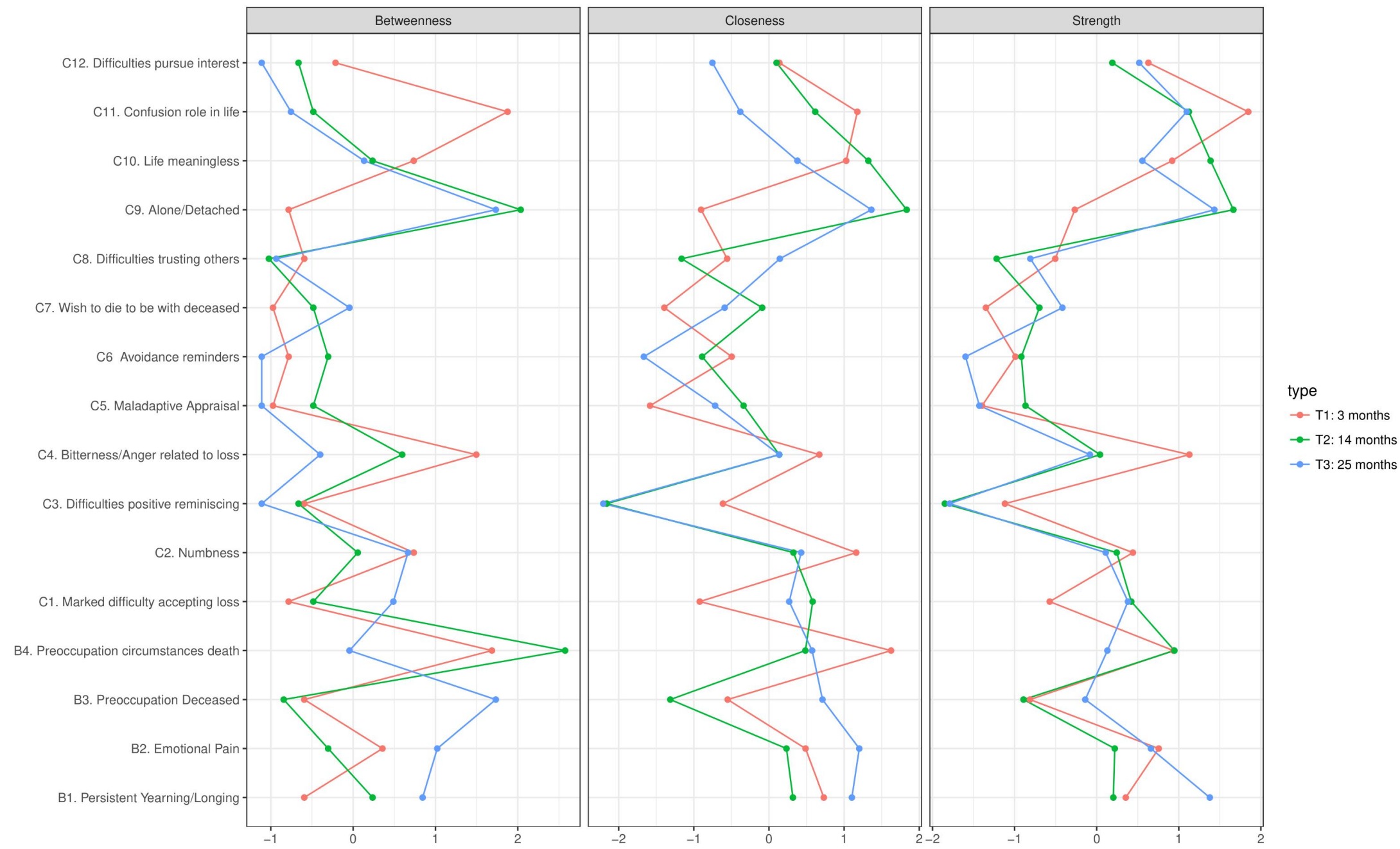
Fig. 2. Comparison of network centrality indexes for symptoms of PCBD at 3 months, 14 months, and 25 months post-loss.
