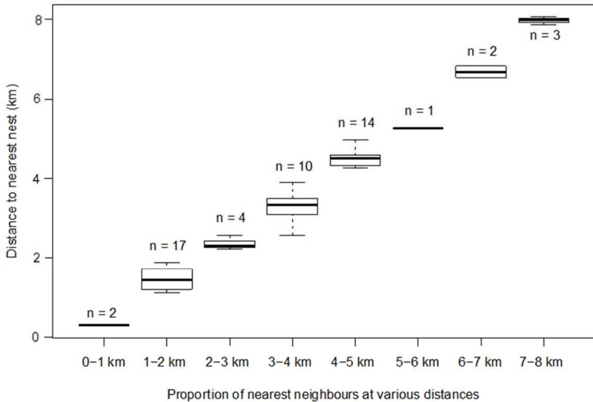
SUPPLEMENTARY FIG. 1 Distances between nearest neighbours among Pallas's fish eagle Haliaeetus leucoryphus nests (n), indicating that most nests are located close to each other and in an aggregated pattern.
