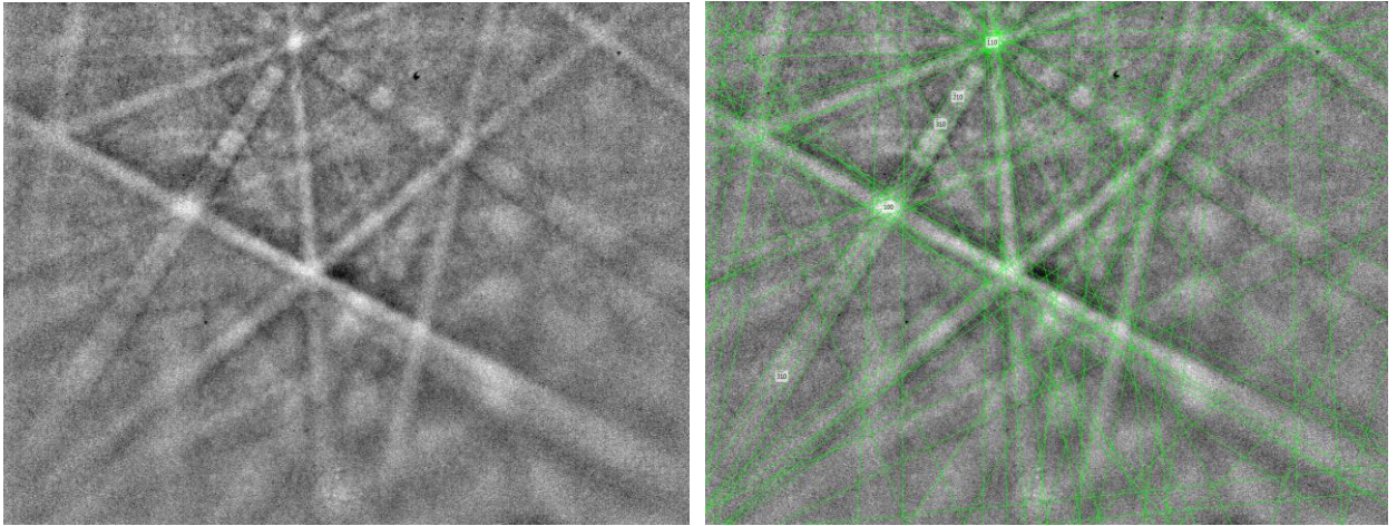
EBSD pattern of mertieite and theoretical mertieite-II (Karimova et al., 2018) solution fit over the pattern with mean angle deviation (MAD) of 0.48^\circ on the basis of maximum of 12 bands.
