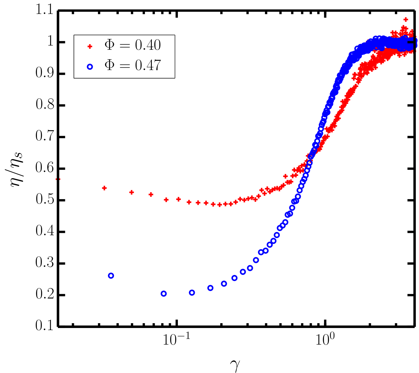
Normalized transient viscosity after shear reversal for different particle volume fractions vs local strain. Local measurements were performed in the middle of the gap (Blanc et al 2011a).
