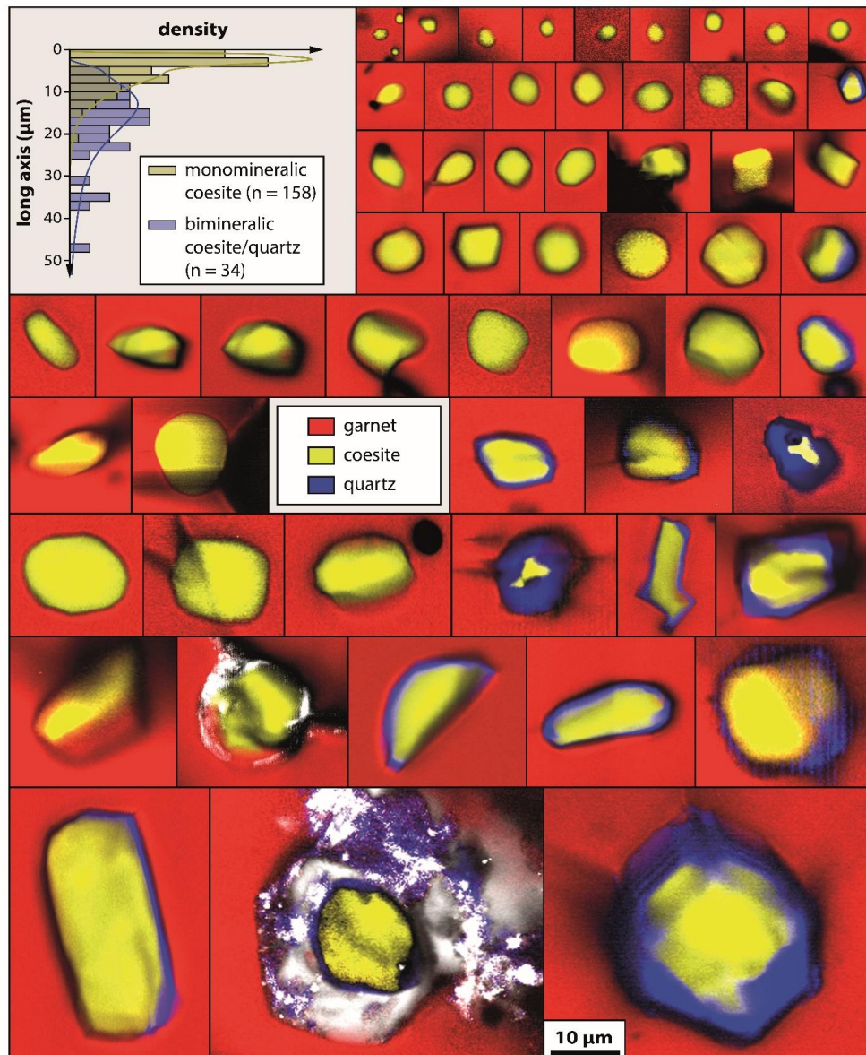
Figure SM4: Monomineralic coesite and bimineralic coesite/quartz inclusions compared to inclusion size. Upper left diagram shows a histogram and kernel density estimates of all coesite inclusions, except one inclusion of sample JS-Erz-9s due to its polyphase character. Two-dimensional Raman images show a selection of coesite inclusions at the same scale ordered with regard to inclusion size. Colors correspond to Raman mode intensities of the garnet (red), coesite (yellow), quartz (blue), and embedding medium (white) components.
