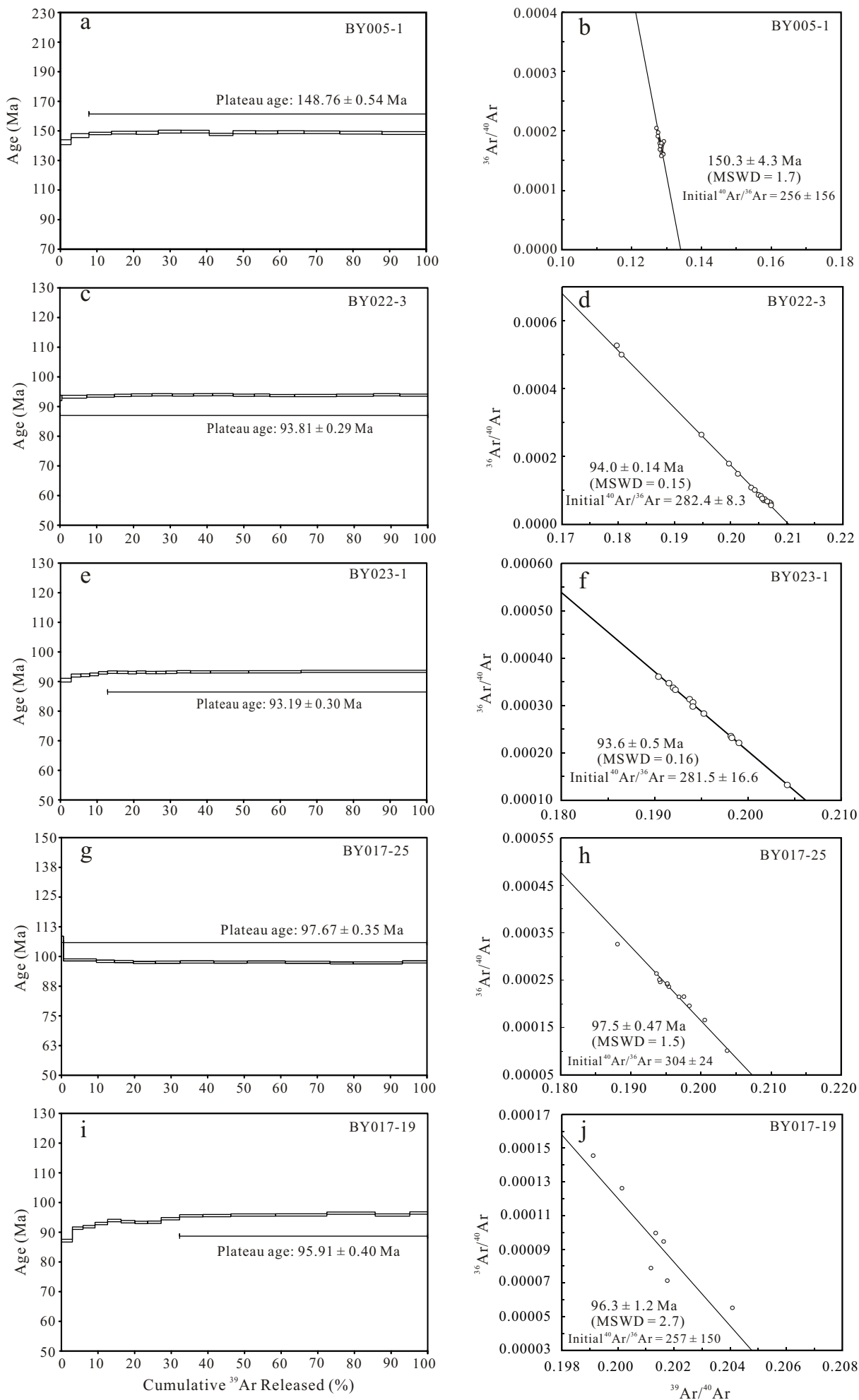
Figure A1. ^{40}\text{Ar} - ^{39}\text{Ar} age spectra and inverse isochrons of biotites from felsic gneisses (BY005-1, BY022-3, BY023-1, and BY017-19) and associated leucosome (BY017-19) in Baiyunshan, with plateau and isochron ages indicated. The heating steps included in the calculations of the inverse isochron age are the same as those in plateau ages.
