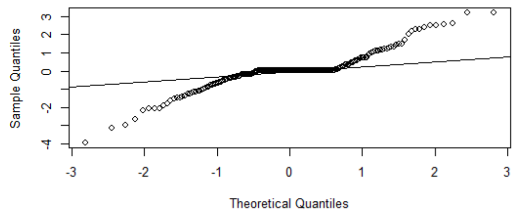
Normal Q-Q Plot of Standardized Residuals
