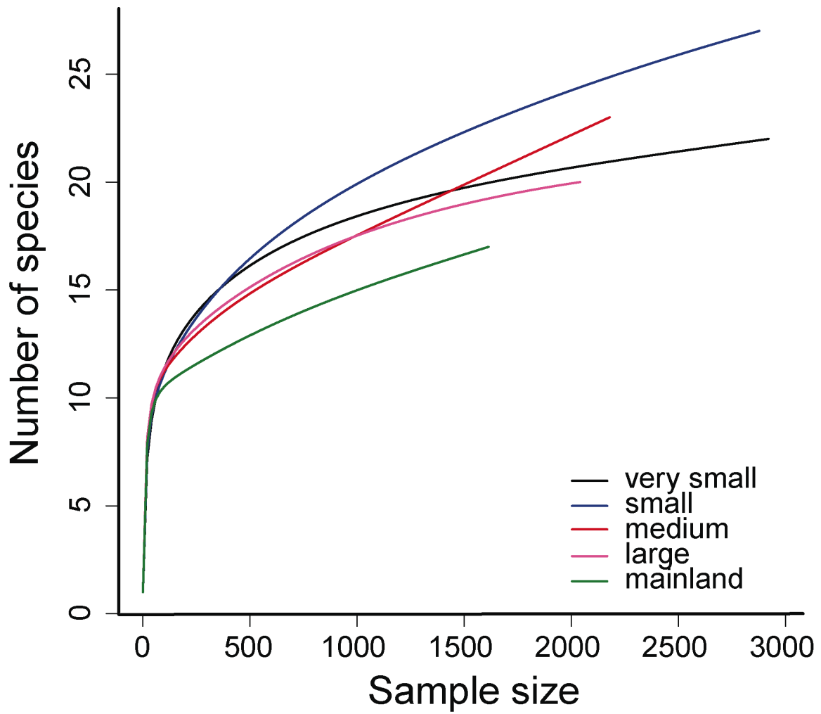
Supplemental Appendix 2. Rarefaction curves illustrating species accumulation for each island class and the mainland.
