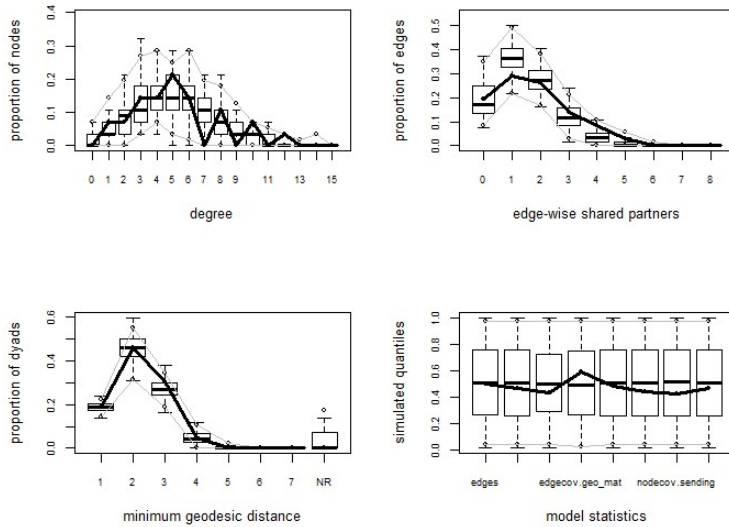
Figure 2. Goodness-of-fit diagnostics for model 2: advice
