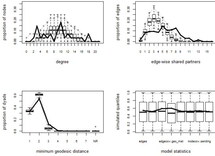
Figure 3. Goodness-of-fit diagnostics for model 3: information
