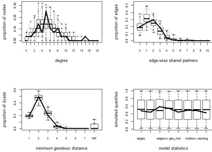
Figure 4. Goodness-of-fit diagnostics for model 4: problem solving
