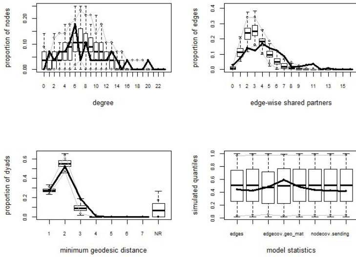
Figure 1. Goodness-of-fit diagnostics for model 1: best practices
