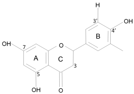
Naringenin
