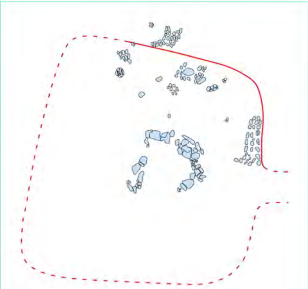
2. unburned rock
