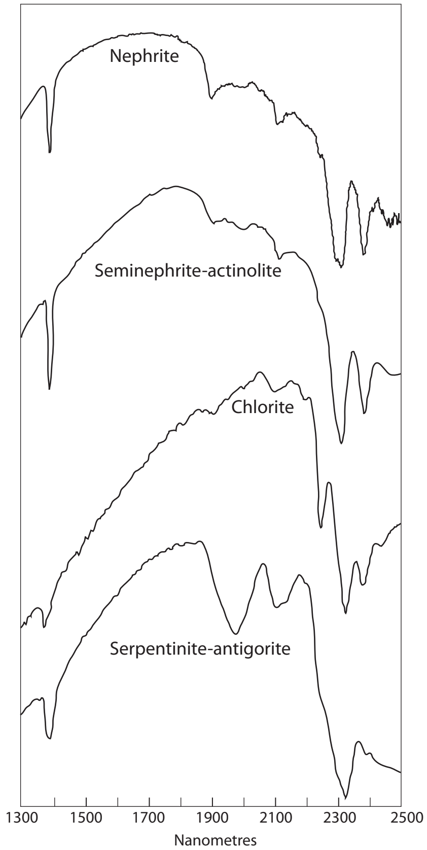
Supplemental Figure 1. NIR spectra of common celt materials.
