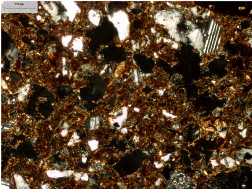
Supplemental Figure 1. Photomicrographs taken at 40X magnification of Type A fabrics. Above, sherd S2-06-45, which contains two of the unweathered feldspar fragments typical of this fabric, photographed in partial cross-polarized light. Below, sherd S3-06-23, photographed in cross-polarized light, which also contains significant quartz and plagioclase feldspar.
