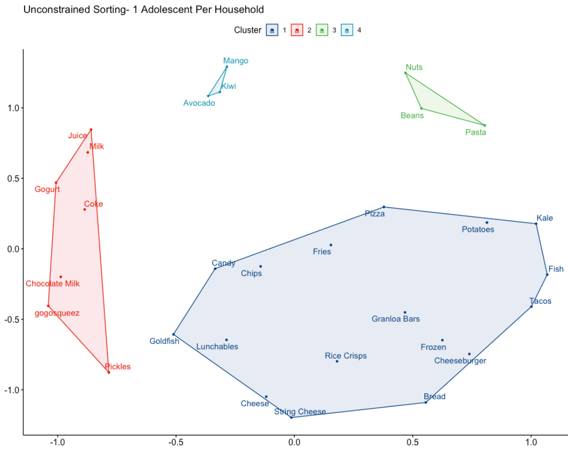
Figure A.2. Multidimensional scaling plot (stress = 0.211) and cluster analysis for one adolescent per household (n=38) unconstrained pilesorts of 30 foods and beverages
