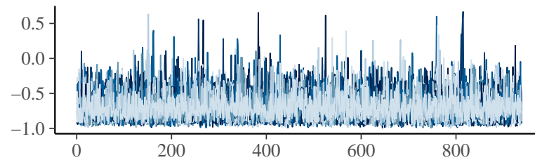
cor_id_ppts_Intercept_cpts_ccseR
