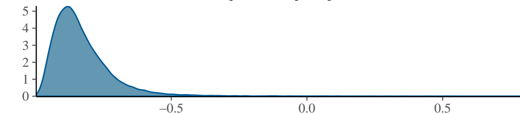
cor_id_cpts_Intercept_cpts_ccseR
