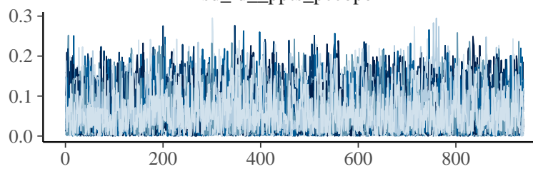
sd_id_ppts_pccopeR
