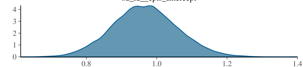
sd_id_cpts_Intercept
