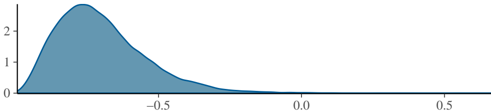
cor_id_ppts_Intercept_cpts_ccseR
