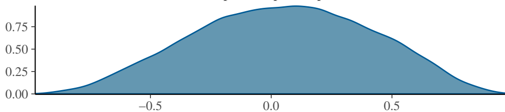
cor_id_cpts_cccopeR_cpts_ccseR
