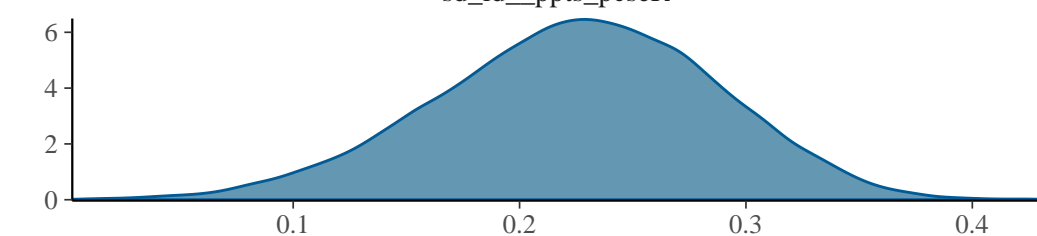
sd_id_ppts_pcseR
