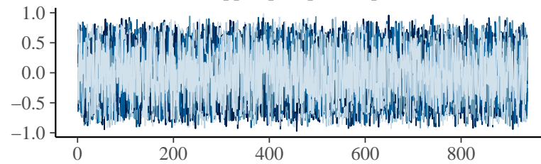
cor_id_ppts_pccopeR_cpts_ccseR
