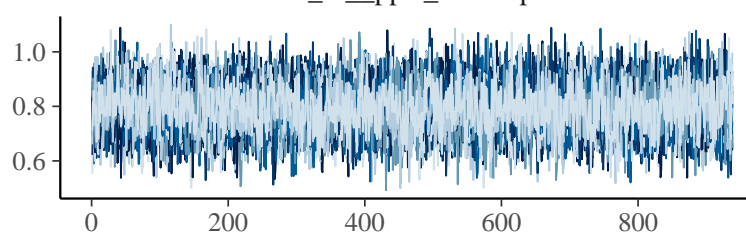
sd_id_ppts_Intercept
