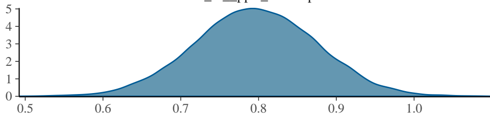
sd_id_ppts_Intercept
