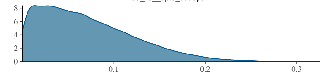
sd_id_cpts_cccpeR
