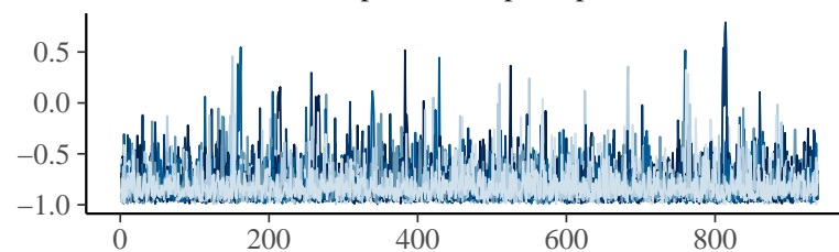
cor_id_cpts_Intercept_cpts_ccseR
