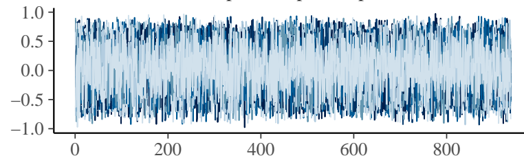
cor_id_cpts_cccopeR_cpts_ccseR
