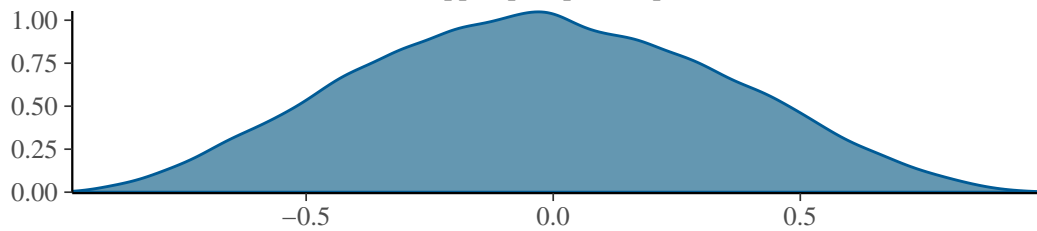
cor_id_ppts_pccopeR_cpts_ccseR
