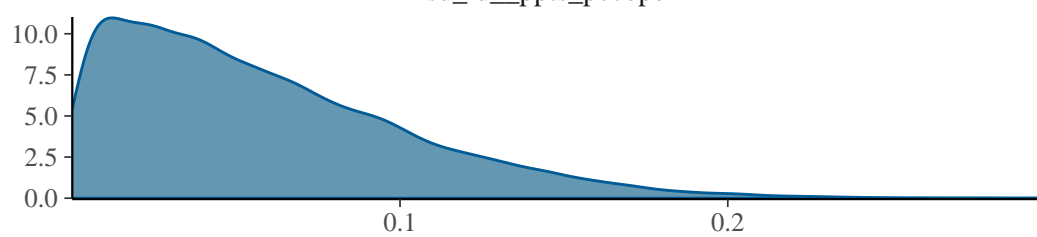
sd_id_ppts_pccopeR
