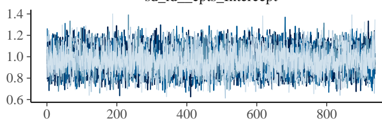
sd_id_cpts_Intercept
