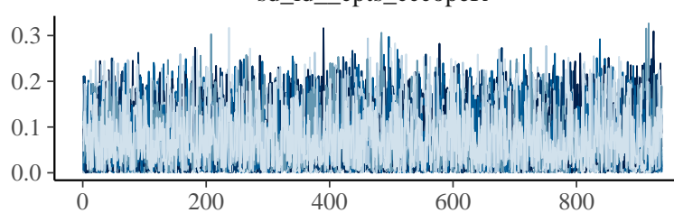
sd_id_cpts_cccpeR
