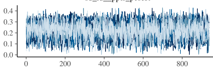
sd_id_ppts_pcseR
