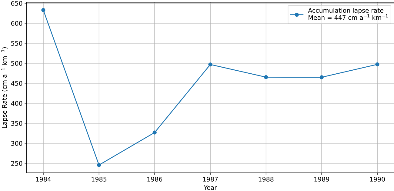
Fig. S9. Seasonal (November to April) accumulation lapse rates calculated between 1984–90. All five stations used had winter snowfall measurements available from 1983/84 to 1989/90.
