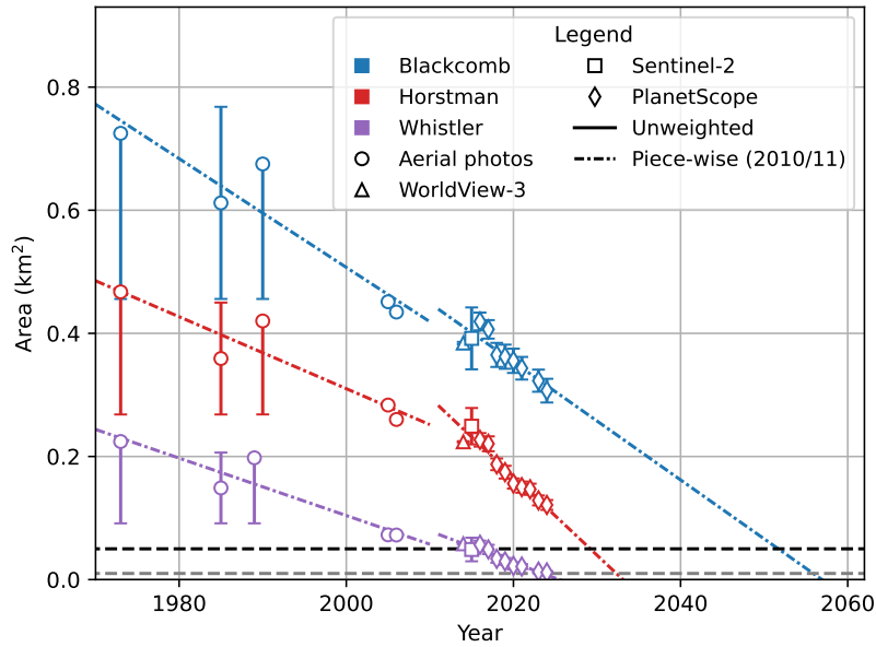
Fig. S5. Timeseries with unweighted and piecewise least-squares linear regressions. Black dashed line indicates the 0.05 \text{ km}^2 threshold (Bolch and others, 2010; Bevington and Menounos, 2022; Peltó and Peltó, 2025) and grey dashed line indicates the 0.01 \text{ km}^2 threshold (Leigh and others, 2019; Maussion and others, 2023). Piecewise regressions split at 2010/11, calculated using data between 1973–2006 and 2014–24. The regressions post-2011 are all steeper than pre-2010, especially for Horstman Glacier. Note asymmetric uncertainties in 1973, 1989, 1990, where snow cover permitted only an upper bound on area.
