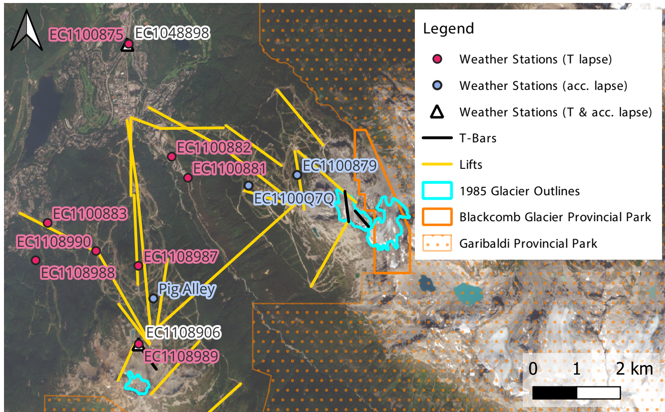
Fig. S7. Overview map showing labelled weather stations. Station names that start with ‘EC’ represent Environment and Climate Change Canada, data obtained via the Pacific Climate Impacts Consortium (2025). Pig Alley weather station data were obtained from the avalanche forecasters on Whistler Mountain in 2025. Stations shown in magenta were used for temperature (T) lapse rate calculations, stations shown in blue were used for accumulation (acc.) lapse rate calculations, and those represented by white triangles were used for both.
