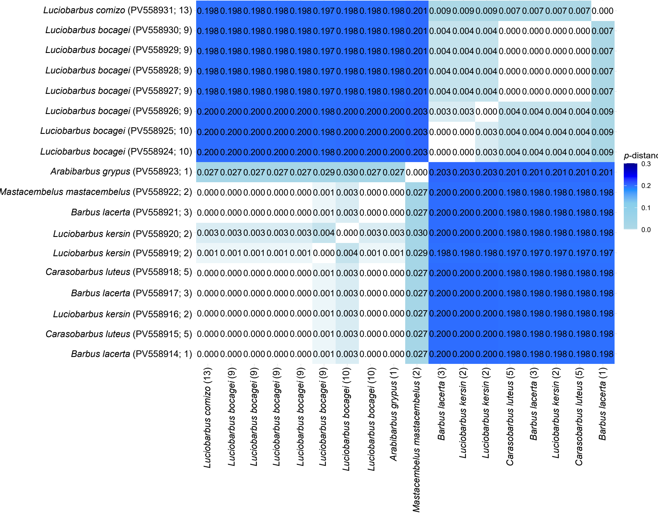
Pair-wise genetic distances in ITS2 (numbers in brackets represent GenBank accession numbers and codes of the localities)
