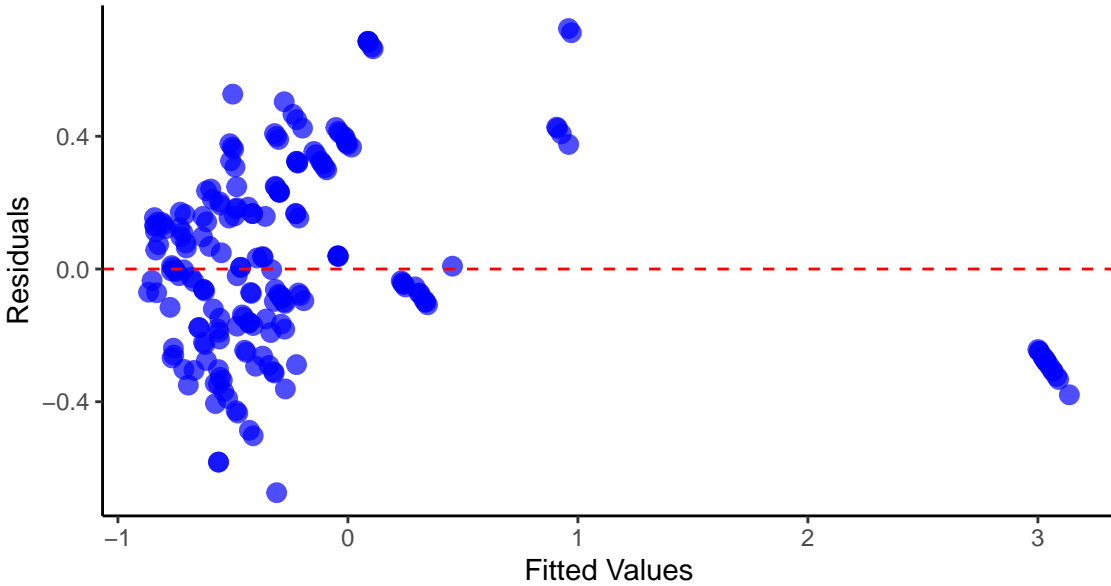
Residuals Plot for model evaluating Haemoproteus diversity
