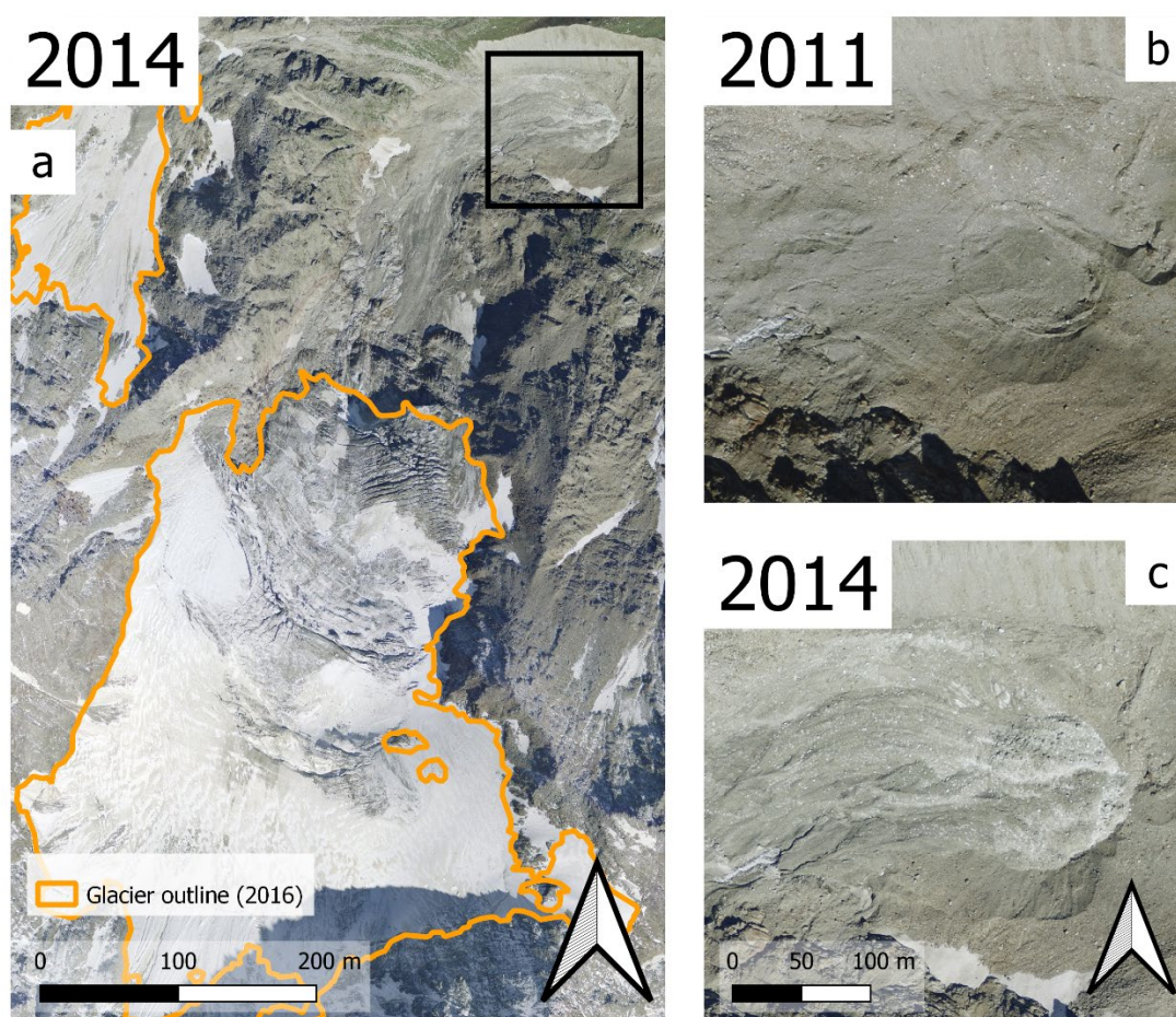
Figure S1: Circular glacier collapse feature at Rossbodegletscher, Switzerland. This is the longest-lived collapse feature in our inventory (28 years lifespan, compared to median lifespan of 4 years). Its longevity could be connected to frequent avalanching. (a): Aerial image of the glacier in 2014, map inset for panels b and c outlined in black. Note that the glacier outline from 2016 no longer includes the lower glacier tongue, after being detached from the upper part of the glacier. (b): Collapse feature in 2011 on the debris-covered glacier tongue. The feature can be identified by the circular crevasses surrounding it. (c): Same map extent as in panel b. An ice avalanche, originating from the remaining glacier to the southwest, deposited ice and snow onto the collapse feature in 2014.
