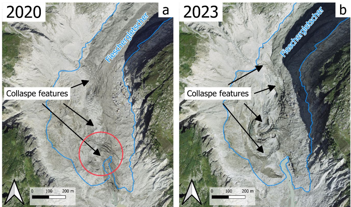
Figure 1: Glacier terminus of Fieschergletscher (Switzerland) in 2020 and 2023. The glacier extent of the year 2022 is shown (blue). The glacier terminus is covered with several collapse features, indicated by circular crevasses. (a): Aerial image of the glacier terminus in 2020. Collapse features are indicated by black arrows. The ice thickness of the southernmost feature (red circle) was found to be 128m at the time of its first appearance (2017). (b): Aerial image of the glacier terminus in 2023. The cavity roof of some features have collapsed, the glacier surface is characterized by many crevasses, ice cliffs and heterogeneous debris cover.
