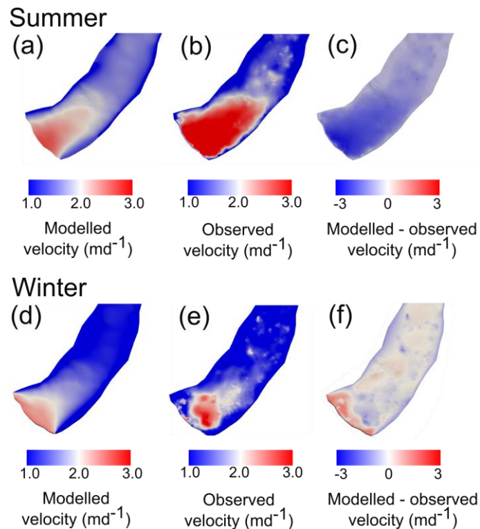
Fig S1: Plots showing the modelled, observed, and modelled-observed velocities during Summer (a-c) and winter (d-f) used for and created by the model inversions
