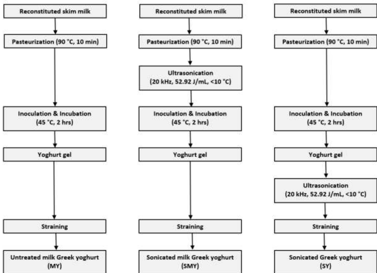
Figure: Process flow chart of Greek yoghurt manufacturing
