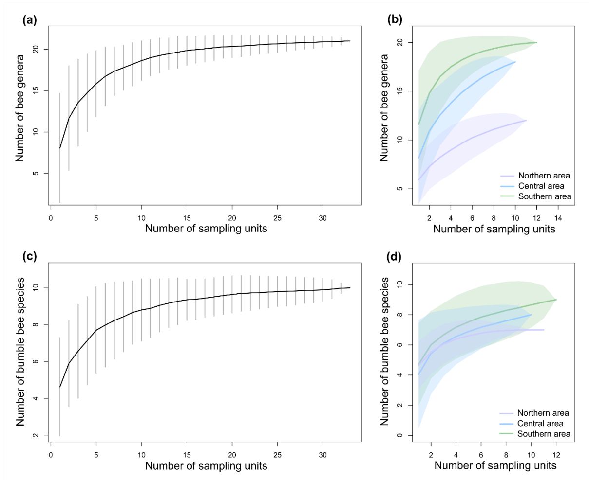
Figure S1. (a) Anthophila genera accumulation curve and its associated standard deviation from n = 999 random permutations of the data for the whole gradient. (b) Anthophila genera accumulation curves (thin solid line) and their associated standard deviation (SD) for the three studied areas along the climatic gradient. (c) Bumble bee species accumulation curve and its associated standard deviation from n = 999 random permutations of the data for the whole gradient. (d) Bumble bee species accumulation curves (thin solid line) and their associated standard deviation (SD) for the three studied areas along the climatic gradient.
