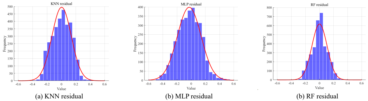
Figure 10. Residual plots of KNN, MLP, and RF algorithms
