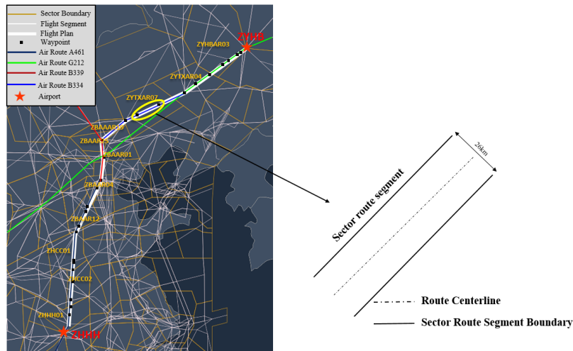
Figure 1. Schematic diagram of sector route segment
