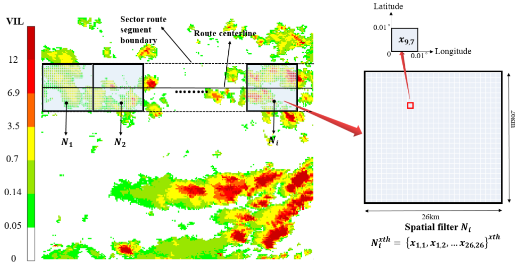
Figure 2. Airspace filter
