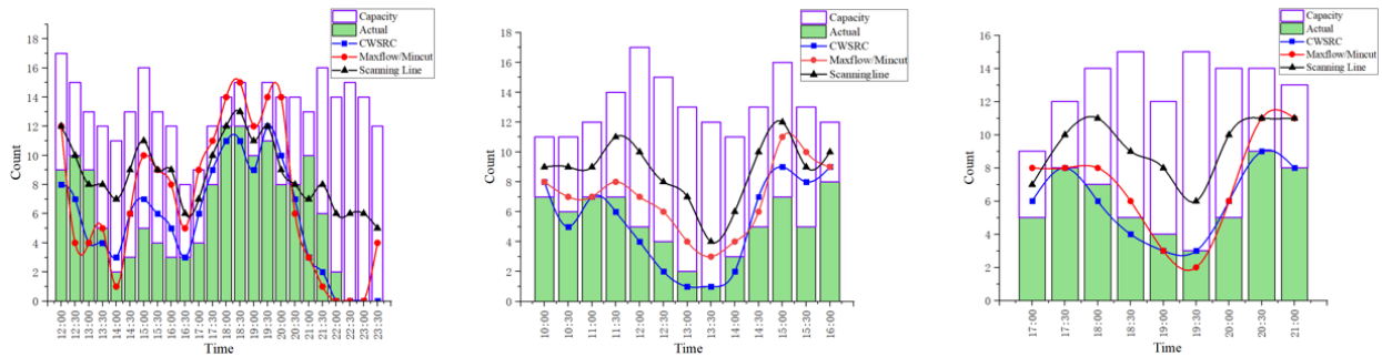
Figure 14. Comparison chart of capacity prediction results for three methods
